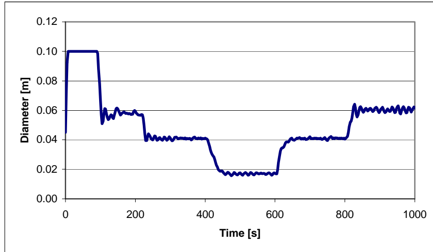
Figure 7: Variation in valve diameter with time.
