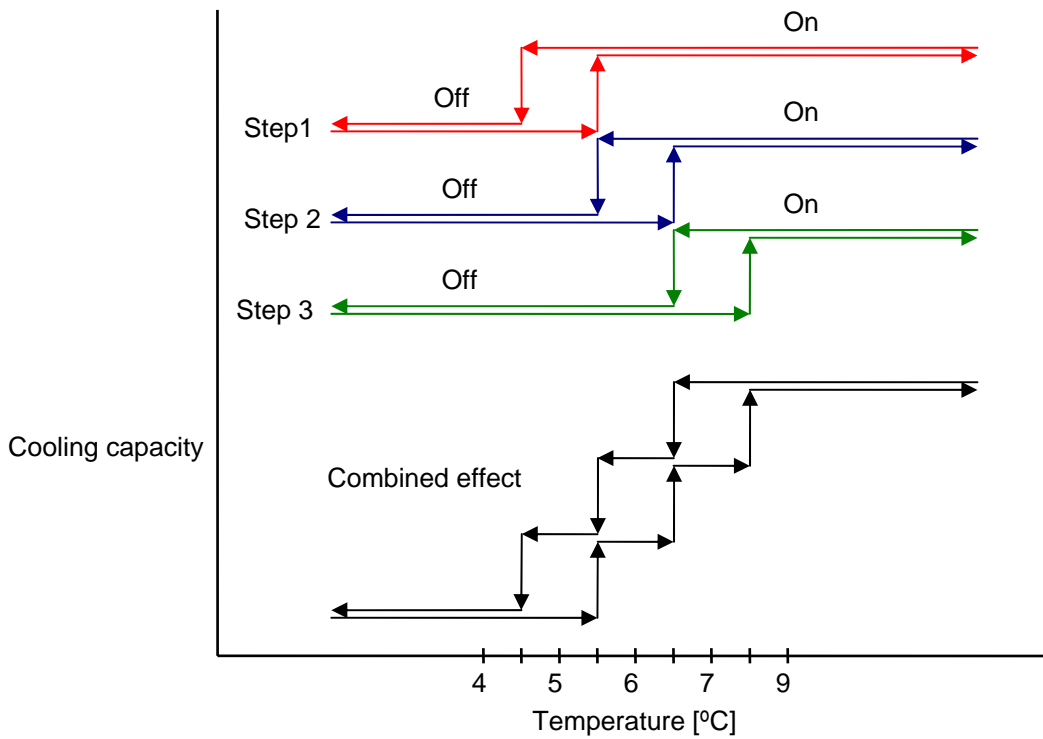
Figure 4: Settings of step controller.
