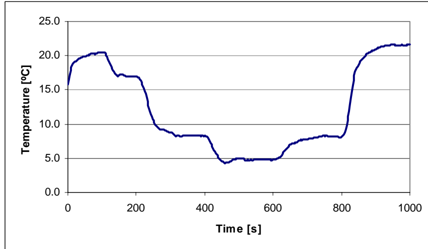
Figure 5: Temperature at inlet to the load with the control valve controller switched off.
