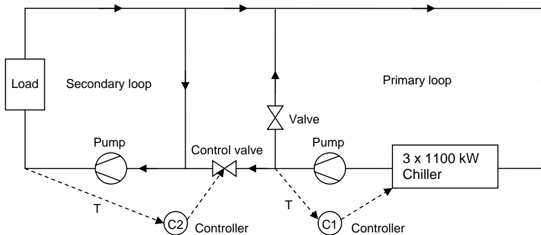
Figure 1: Layout of three-step chiller plant.
