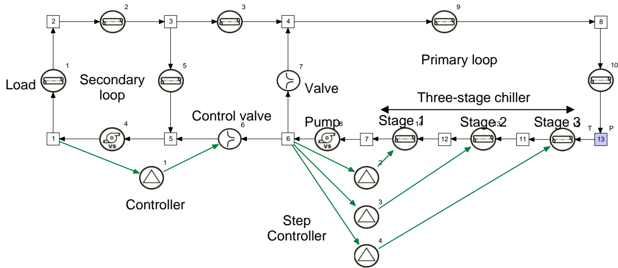
Figure 2: Flownex model of the three stage chiller plant with control system.
