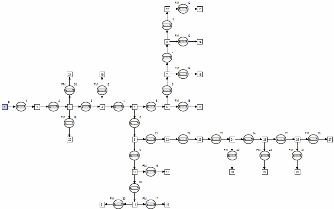
Figure 2: Flownex network.
